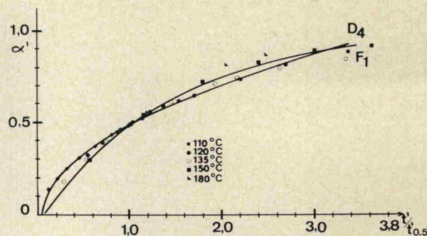
Fig. 2. Reduced time representation, after correction for adsorbed water, for isothermal decomposition of \gamma\text{-FeOOH} . The data used are a set different from that in fig. 1. Two calculated curves for different mechanism models from fig. 7 are also shown. \alpha' = corrected reaction rate from 0 to 1 (or 0 to 100%)
